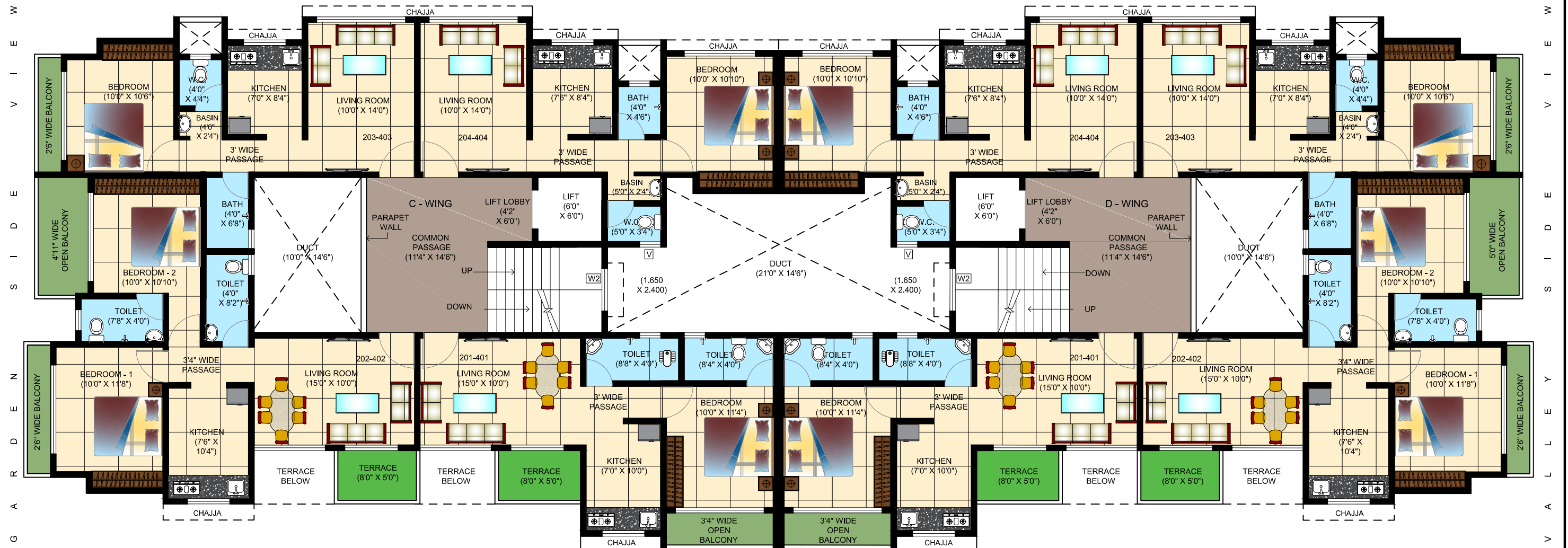
SECOND & FOURTH FLOOR PLAN C-WING & D - WING
