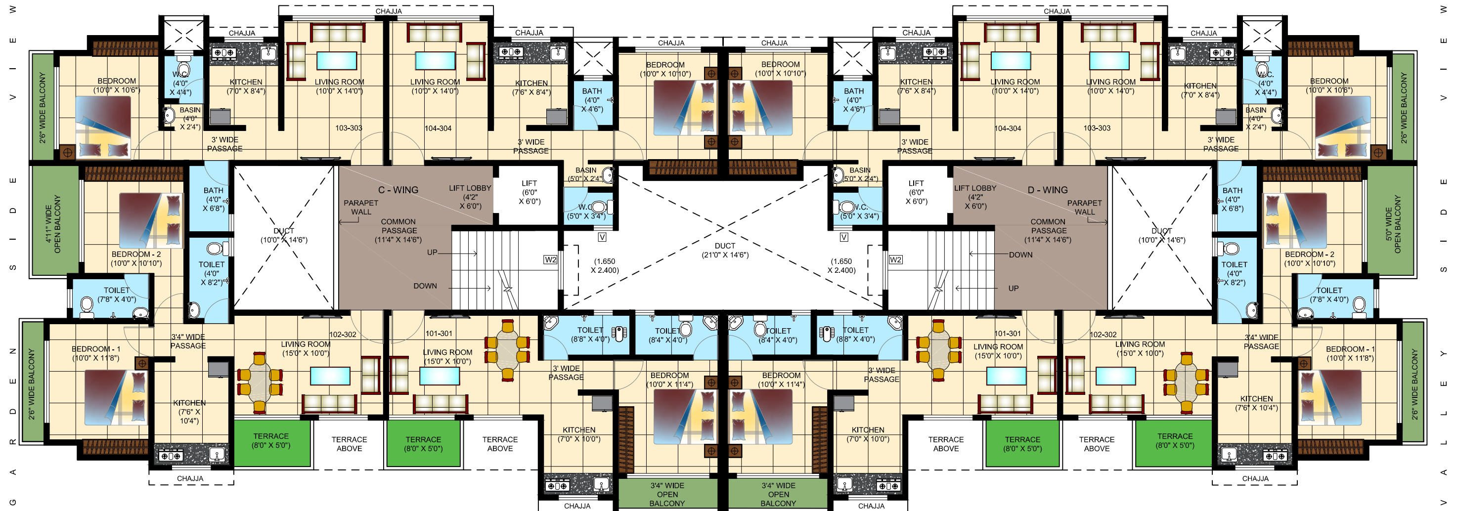
FIRST & THIRD FLOOR PLAN C-WING & D - WING
